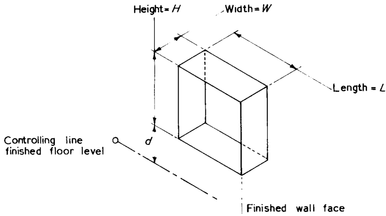
Figure 4. Explanation of dimensions (for further details see figure 3)
