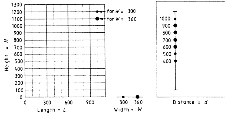
Figure 5. Co-ordinating spaces for fixed hose reels Delete the existing drawing and substitute the following drawing.
