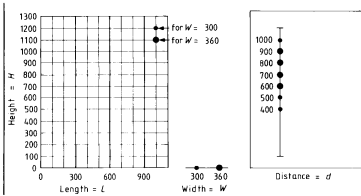
Figure 5. Co-ordinating spaces for fixed hose reels (see also 14.2)
