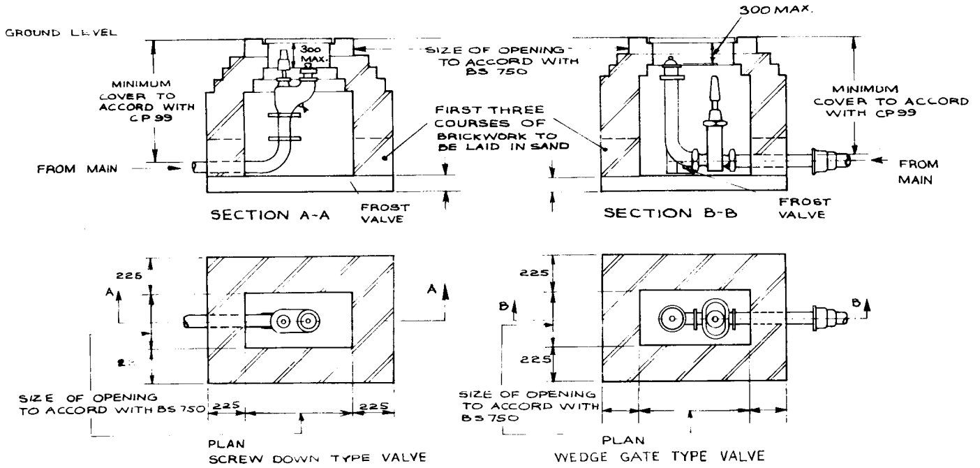
Figure 1. Typical layout of pit for underground fire hydrant (brick)
